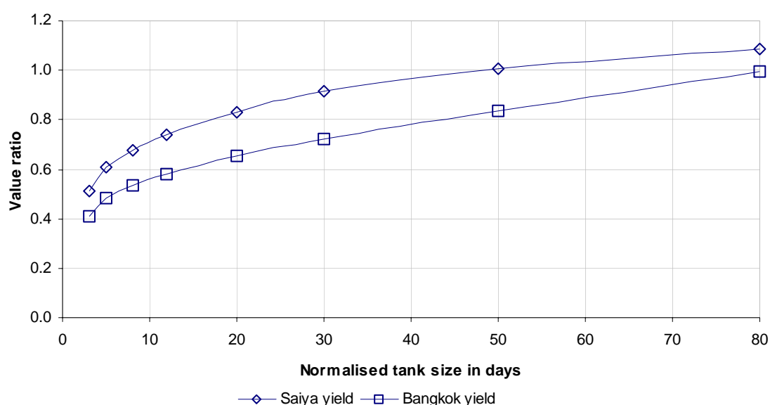
Figure 4: Diminishing returns with increase in tank size
