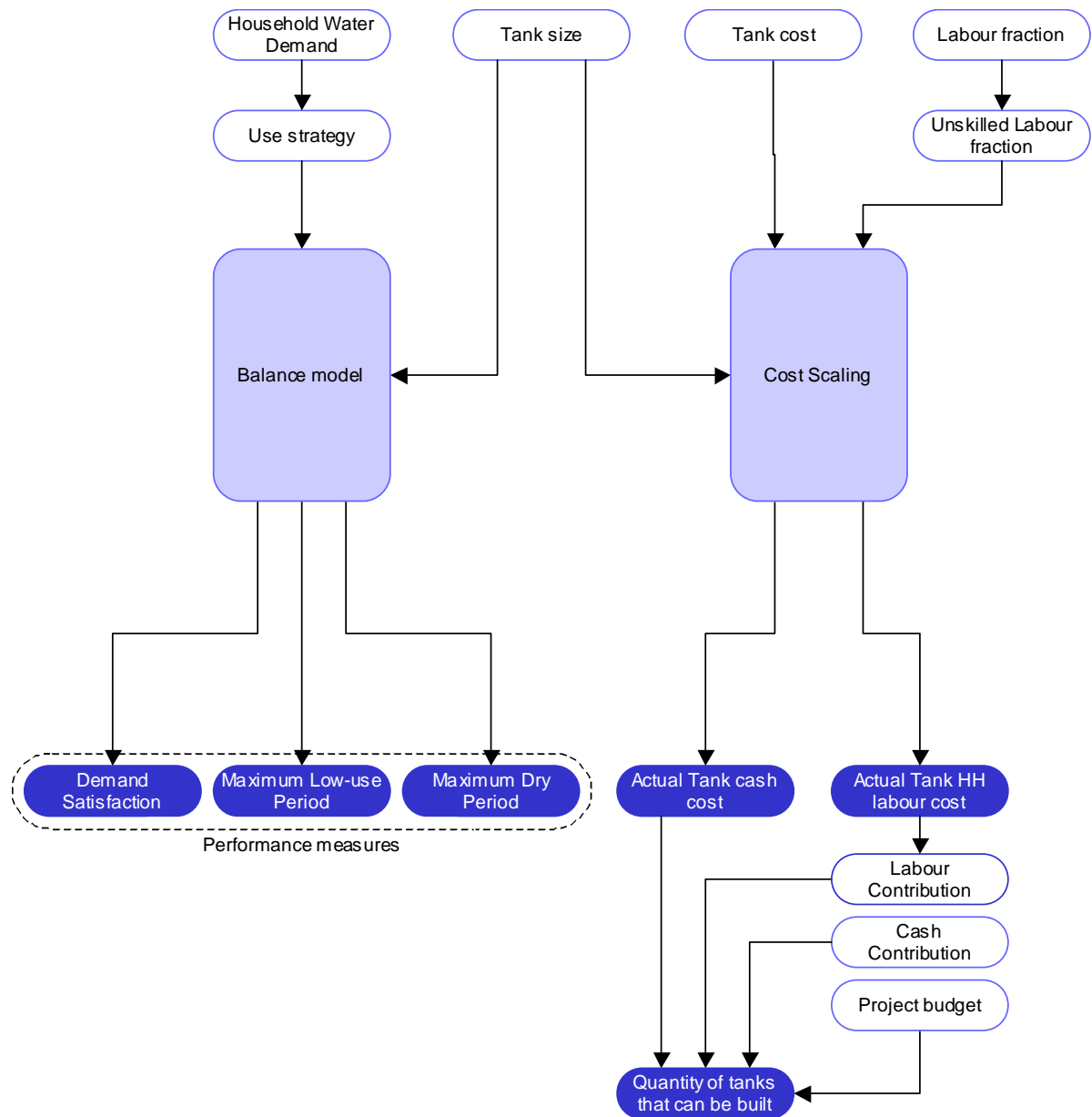
Figure 6: Steps to produce a roofwater harvesting ladder
