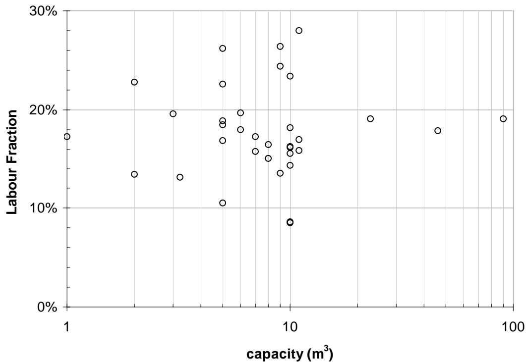
Figure 8: Labour content of construction costs (based on bills of materials and Ugandan cost data)
