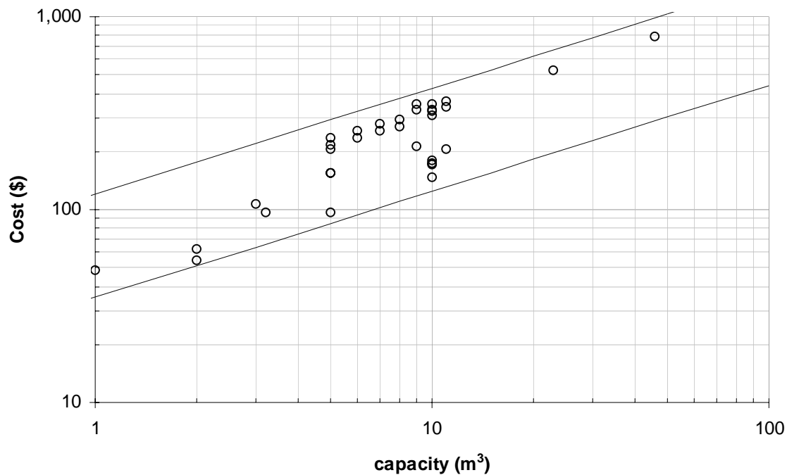
Figure 7: Tank costs (based on bills of materials and Ugandan cost data in 2002)
