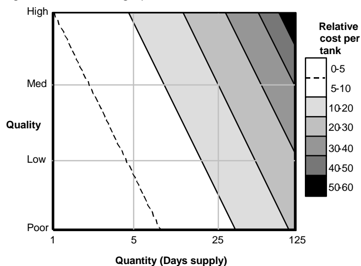
Figure 1: Schematic graph of cistern cost versus size and construction quality.
