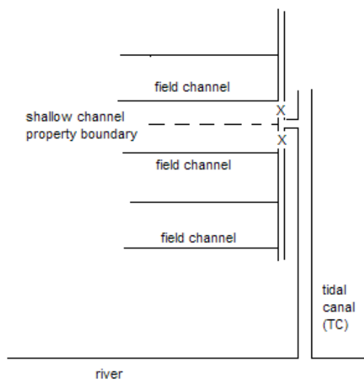
Figure 13. Layout Type 2 with property boundary and two gates
