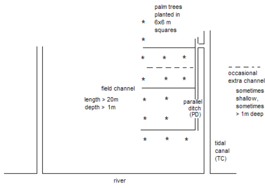
Figure 10. Type 2 layout of tidal irrigation system
