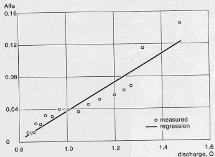
Figure 1 Comparison of \alpha with measured and calculated discharge values
